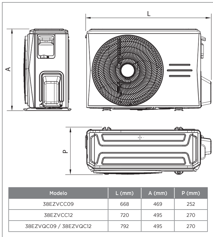
FIG. 4 - DIMENSIONAL
